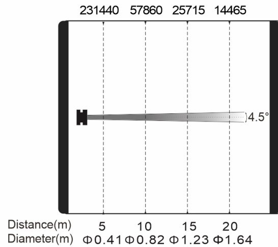
Intensity LUX (4.5°)
